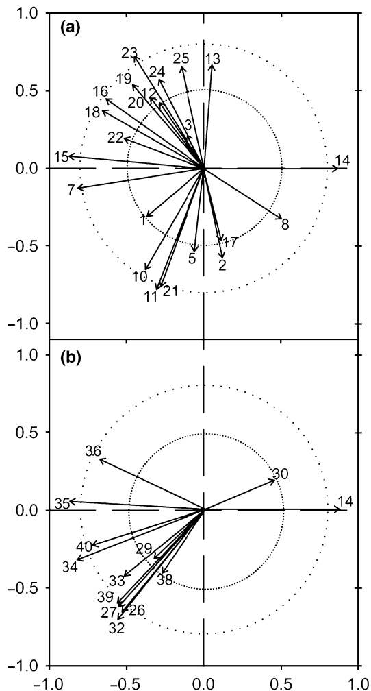
Fig. 2 Loading plots associated with the nonmetric multidimensional scaling (NMDS) ordination in Fig. 1 for (a) monoterpene; (b) sesquiterpene components of oil from Eucalyptus polybractea . Each line represents the direction of the line of best fit for the relevant component of the oil (see Table 1 for component names) within the ordination. The length of the line is equal to the regression coefficient ( r ) of the component data along that line, and is indicative of how strongly that component influenced the ordination. Dotted circles, r values of 0.5 and 0.8.
