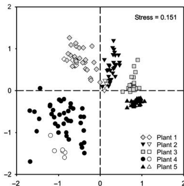
Fig. 1 Nonmetric multidimensional scaling (NMDS) ordination of oil-composition data from individual oil glands (closed symbols) and leaf extracts (open symbols) of five plants of Eucalyptus polybractea corresponding to those in Table 1. The stress of the ordination is 0.151.
